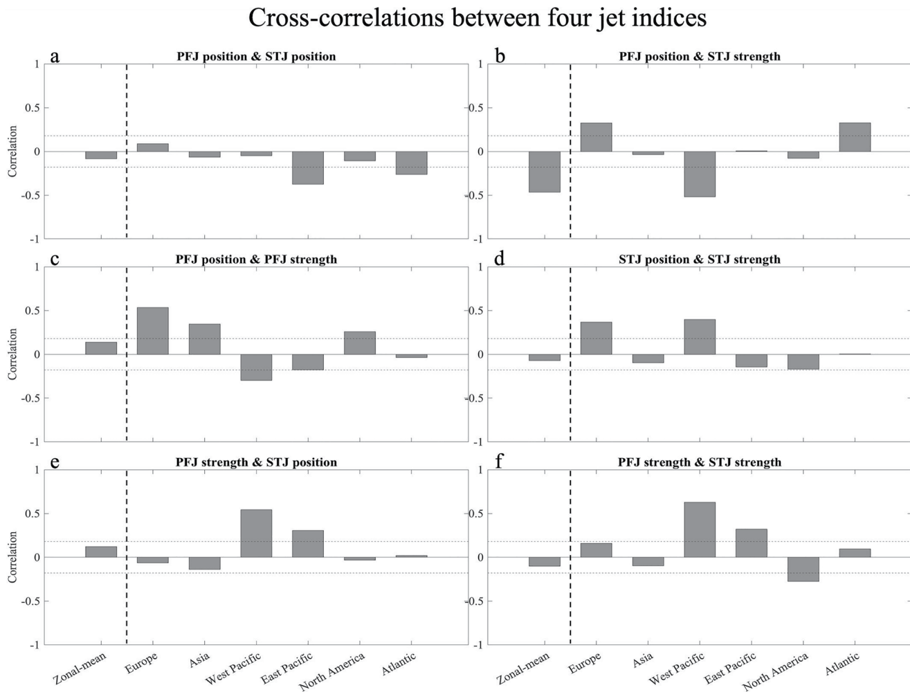
Figure 2. Correlations between monthly time series of the positions and strengths of the PFJ and STJ during NH winter, based on ERA-Interim reanalysis (1979–2018). The jets are defined in the zonal-mean and for the six different regions defined in Section 2.2. The seasonal cycle is removed prior to the analysis. The horizontal dashed lines in each panel indicate the minimum value for significant correlations at the 95% confidence level according to a two-tailed Student's t test.
