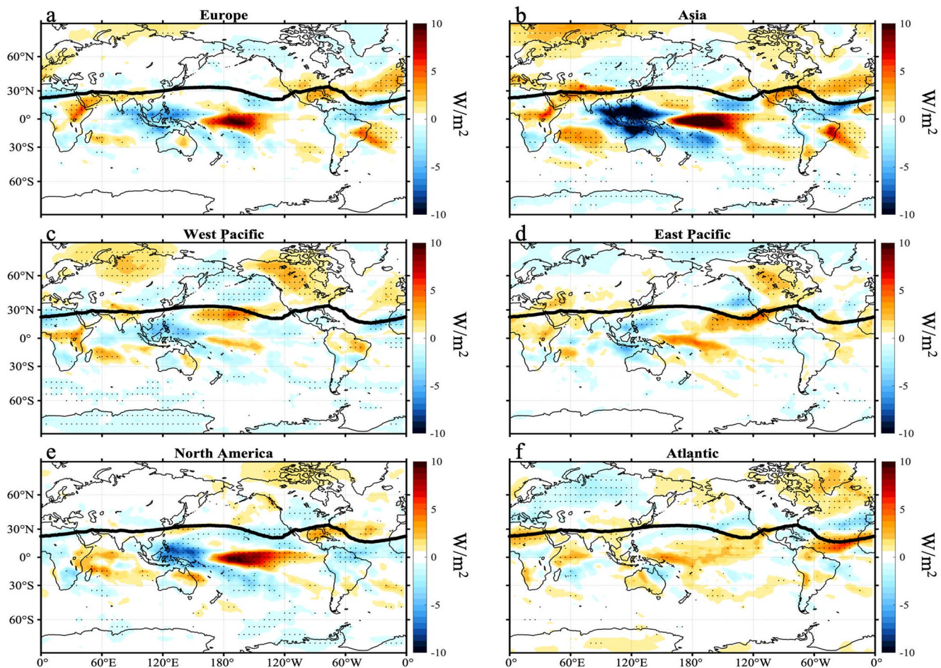
Figure 6. Regression of wintertime monthly outgoing longwave radiation (OLR) anomalies onto six different regions' subtropical jet position in observations. Patterns correspond to OLR anomalies associated with a one standard deviation of poleward shift of the STJ in each region. Thick black lines on each panel are climatological STJ positions in observations as shown in Figure 1a. Stippling indicates that regression patterns are statistically significant at the 95% level according to a two-tailed Student's t test. The model version of this figure is shown in Figure S8 in Supporting Information S1.
