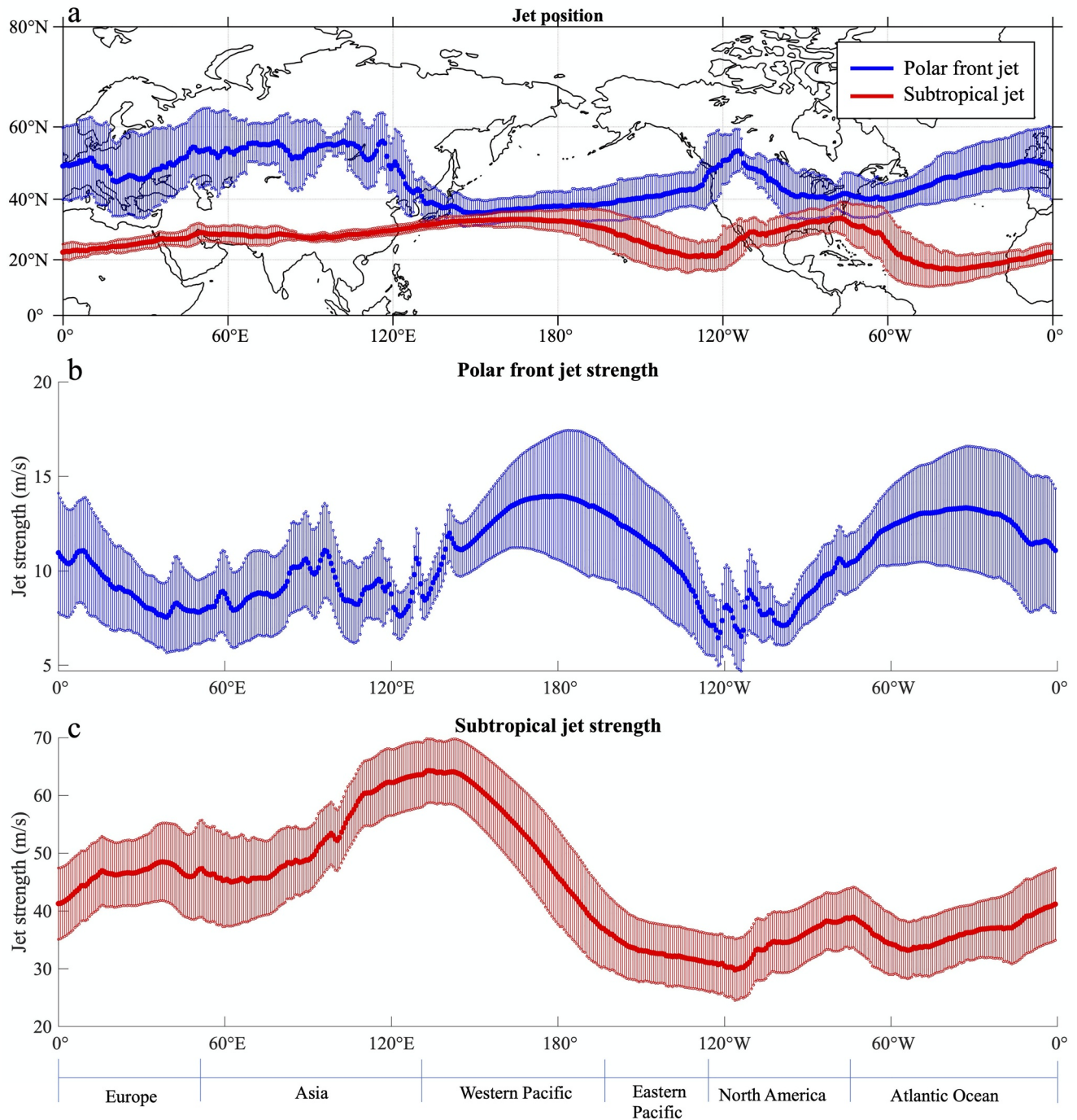
Figure 1. Mean positions (a) and strengths (b, c) of the Northern Hemisphere (NH) wintertime (December–February) PFJ and STJ with \pm 1 standard deviation (shading) shown at all longitudes using jet indices derived from the ERA-Interim reanalysis data set from 1979 to 2018. Note that the jet strengths in panels (b) and (c) are plotted on different scales. The polar front jet is defined using the 850 hPa zonal wind, whereas the subtropical jet is defined using the 250–850 hPa difference in zonal winds.
