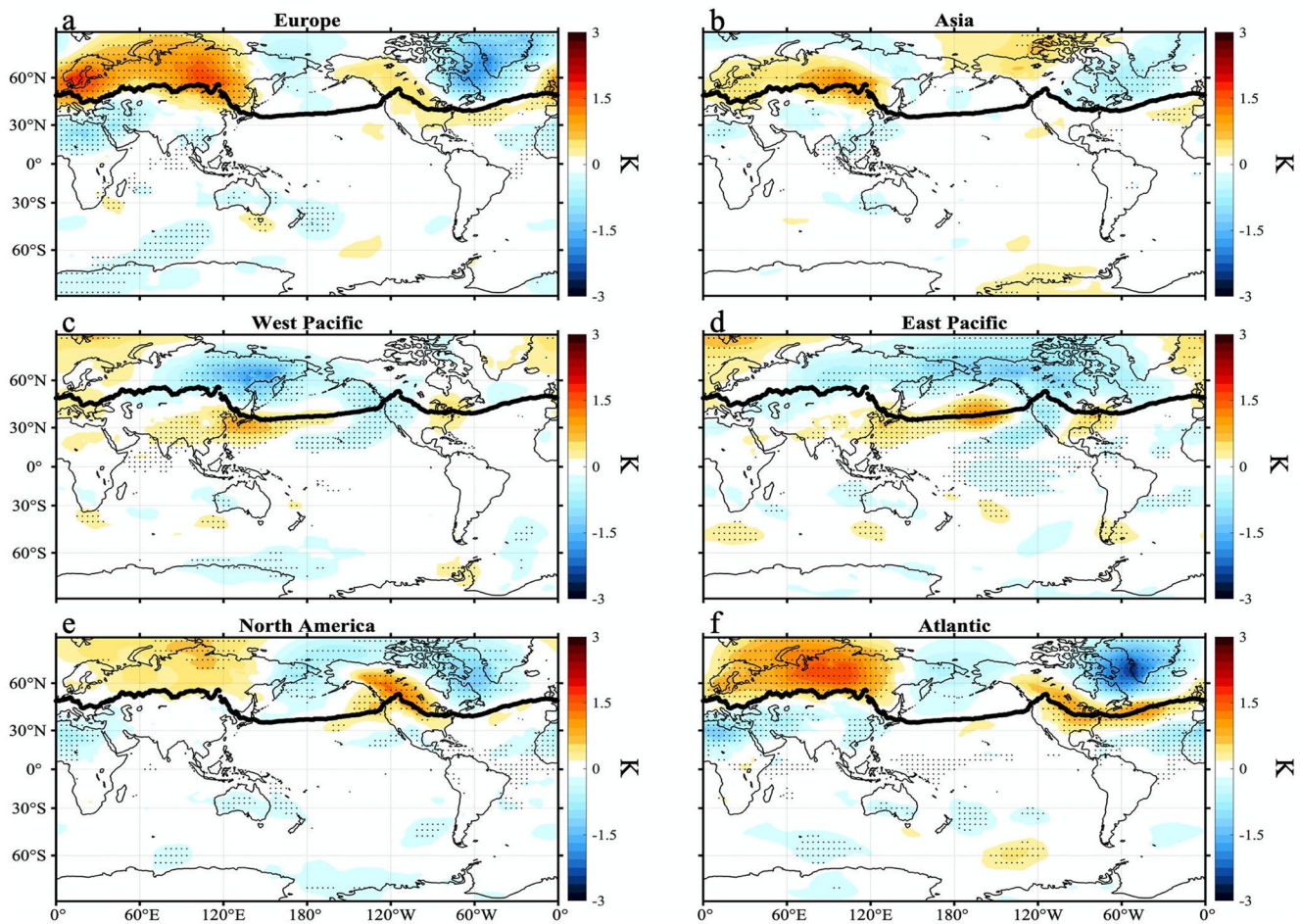
Figure 3. Regression of wintertime monthly 850 hPa temperature anomalies onto six different regions' polar front jet position in observations. Patterns correspond to 850 hPa temperature anomalies associated with a one standard deviation poleward shift of the PFJ in each region. Thick black lines on each panel are climatological PFJ positions in observations as shown in Figure 1a. Stippling indicates that regression patterns are statistically significant at the 95% level according to a two-tailed Student's t test. The model version of this figure is shown in Figure S1 in Supporting Information S1.
