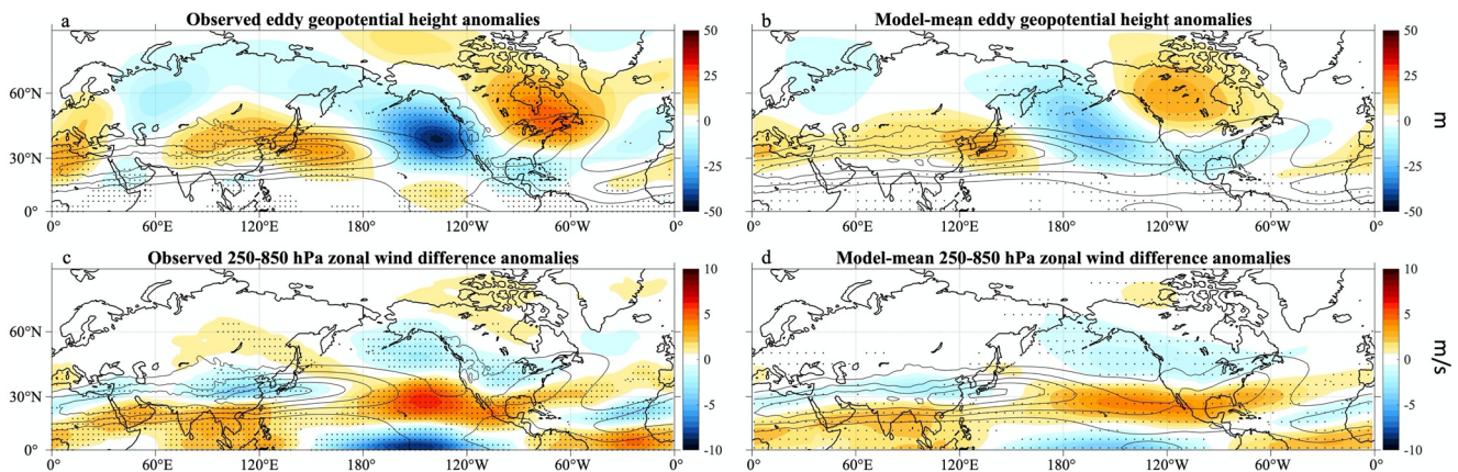
Figure 12. Regression of wintertime monthly eddy 500 hPa geopotential height anomalies (i.e., with both the seasonal cycle and zonal-mean field removed) and 250–850 hPa zonal wind difference anomalies onto the Niño 3.4 index in observations (a, c) and the CMIP6 multimodel-mean panels (b, d). Stippling in panels (a) and (c) indicates that regression patterns are statistically significant at the 95% level according to a two-tailed Student's t test, and stippling in panels (b) and (d) indicates that more than 80% of models agree with the sign of regression coefficients. Black contours indicate the climatology of zonal wind difference field (250 hPa zonal wind–850 hPa zonal wind), which is used to define the STJ position. Contours are shown at 20, 30, 40, 50, and 60 m/s.
