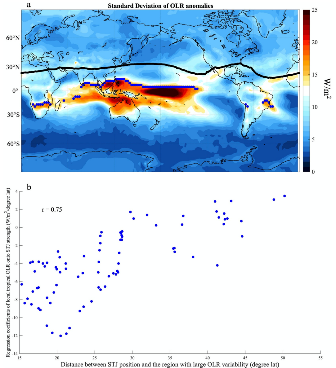
Figure 9. (a) Month-to-month standard deviation of OLR anomalies within DJF season (seasonal cycle removed). Thick black line is climatological STJ position in observations as shown in Figure 1a. The north boundary of the region with large OLR variability is defined as the first latitude where the standard deviation of OLR is greater than 16\ W\ m^{-2} and is denoted as a blue dot at each longitude. (b) Scatter plot between the regression coefficients of local tropical OLR onto STJ strength (i.e., the values along the diagonal of Figure 8c) and the distances between STJ position and the region with large OLR variability across all longitudes in observations (i.e., distance between the black line and the blue dots at all longitudes).
