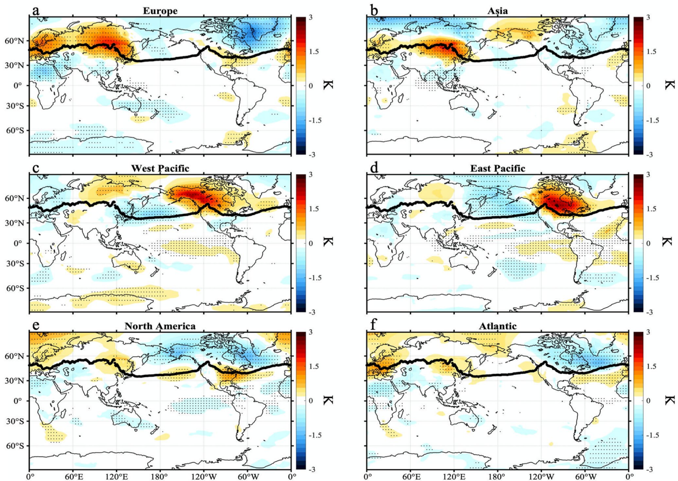
Figure 5. As in Figure 3, but for the PFJ strength. The model version of this figure is shown in Figure S2 in Supporting Information S1.
