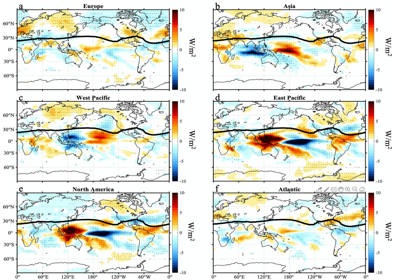
Figure 7. As in Figure 6, but for STJ strength. The model version of this figure is shown in Figure S9 in Supporting Information S1.
