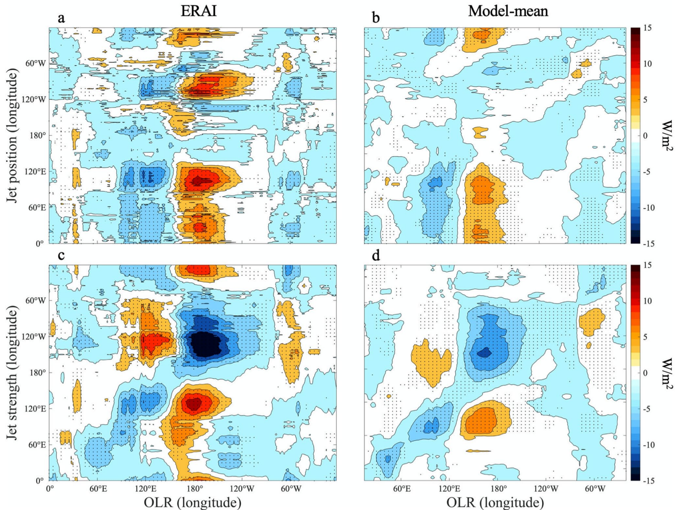
Figure 8. Regression of the wintertime monthly tropical OLR anomalies at the Equator onto subtropical jet indices at all longitudes. (a, b) Regression coefficients for subtropical jet position; (c, d) Regression coefficients for subtropical jet strength. The left column shows results for observations, and the right column shows results for the CMIP6 multimodel-mean. Color shading represents the regression coefficient of OLR at the longitude on the x-axis to the subtropical jet index at the longitude on y-axis. For panels (a) and (c), stippling indicates that regression patterns are statistically significant at the 95% level according to a two-tailed Student's t test. For panels (b) and (d), stippling indicates that more than 80% of models agree on the sign of the regression coefficients.
