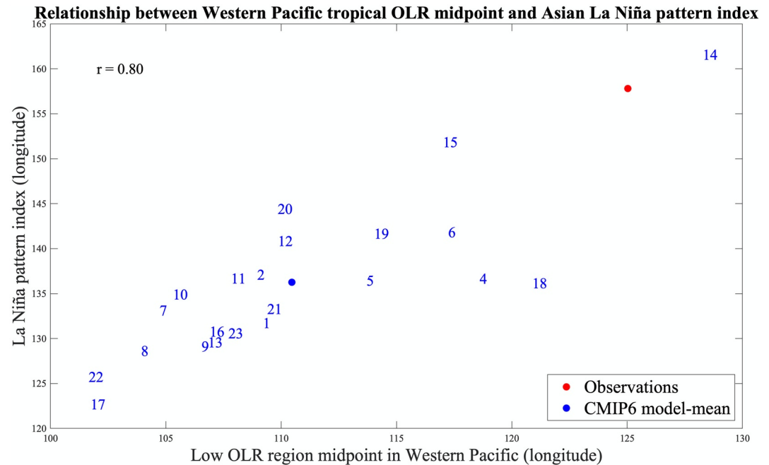
Figure 11. Scatter plot between the midpoint of the wintertime climatological low OLR region over the western Pacific and the La Niña pattern index. The La Niña pattern index is defined as the transition longitude between 120°E and 180°E where the regression coefficient of wintertime monthly OLR anomalies to the Asian STJ position (as shown in Figures 10a and 10b) averaged over 10°S–20°N crosses zero. The midpoint of the climatological low OLR region is defined as the midpoint longitude of the low OLR region in equatorial western Pacific (as shown in Figure 10e). The low OLR region is defined where the OLR is smaller than 255 \text{ W m}^{-2} . Numbers on the scatterplot correspond to the models listed in Table S1 in Supporting Information S1. The blue dot represents multimodel-mean, while the red dot is for observations.
