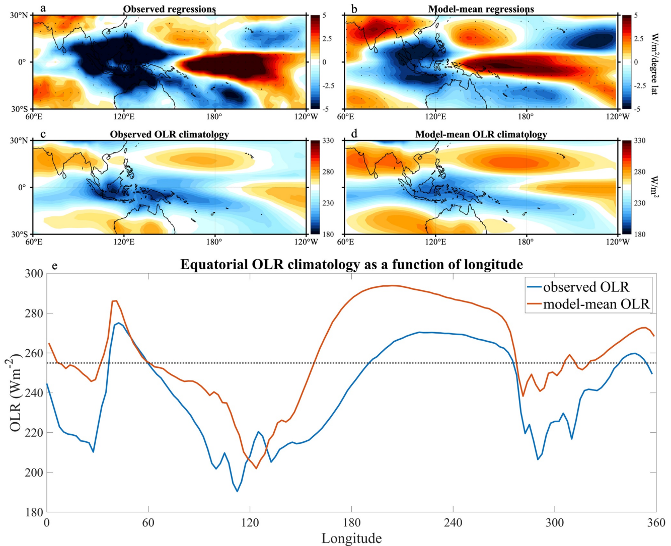
Figure 10. (a, b) Regressions of monthly wintertime OLR anomalies to the Asian STJ position for observations and the CMIP6 multimodel-mean (reproduced from the second panels of Figure 6 and Figure S8 in Supporting Information S1 but zoomed in and with different color scales). (c, d) The wintertime OLR climatology for observations and the CMIP6 multimodel-mean. (e) The observed and multimodel-mean wintertime OLR climatology at the Equator as a function of longitude. The blue line shows the observed OLR, while the red line shows the model-mean OLR. The dashed black line shows the 255 W m -2 OLR value, below which is defined as low OLR.
