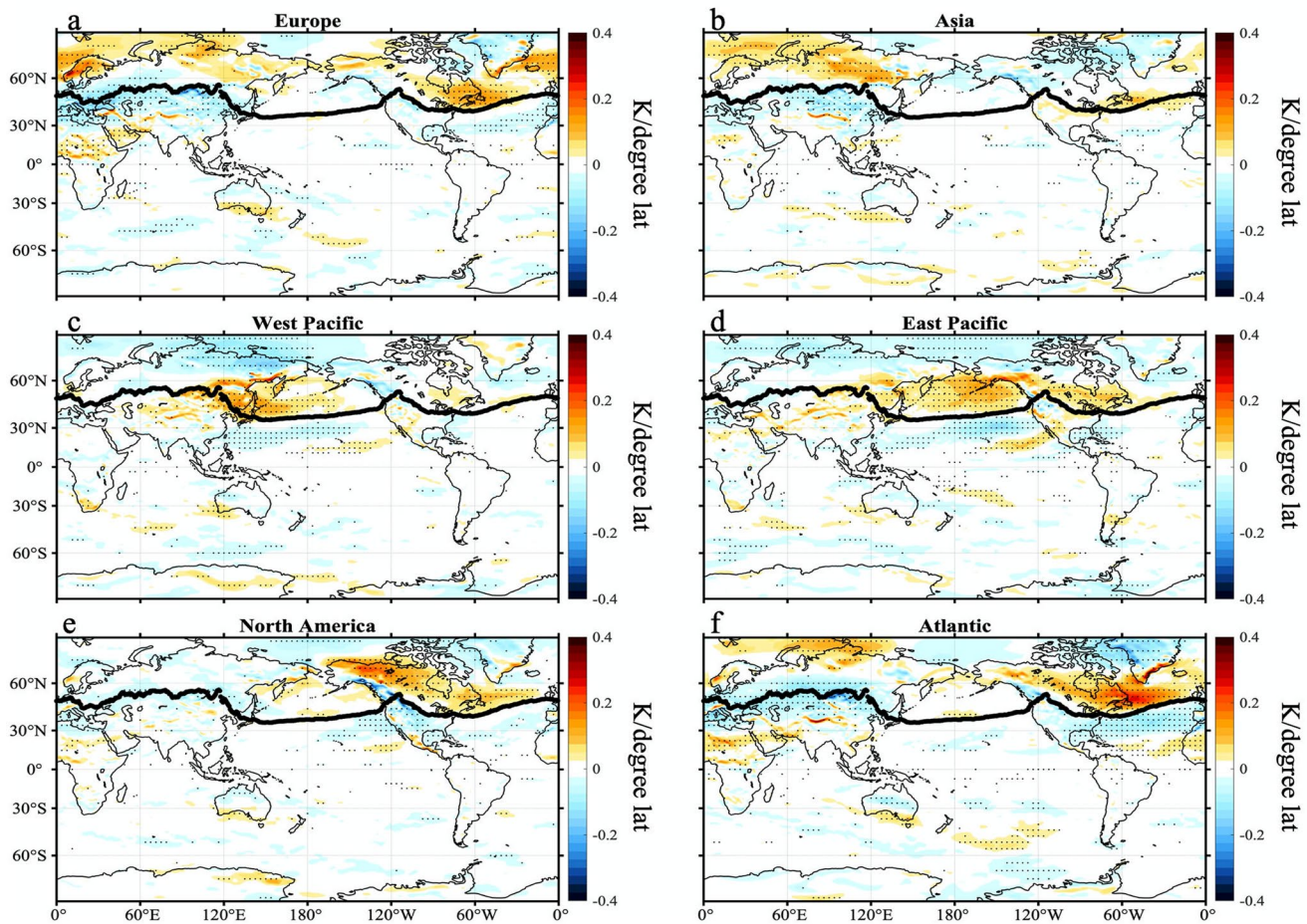
Figure 4. Regression of wintertime monthly 850 hPa meridional temperature gradient anomalies onto six different regions' polar front jet position in observations. Patterns correspond to 850 hPa meridional temperature gradient anomalies (K per degree latitude) associated with a one standard deviation poleward shift of the PFJ in each region. These 850 hPa meridional temperature gradient anomalies are calculated from south to north; therefore, red regions indicate an increase of the meridional temperature gradient. Thick black lines on each panel are climatological PFJ positions in observations as shown in Figure 1a. Stippling indicates that regression patterns are statistically significant at the 95% level according to a two-tailed Student's t test.
